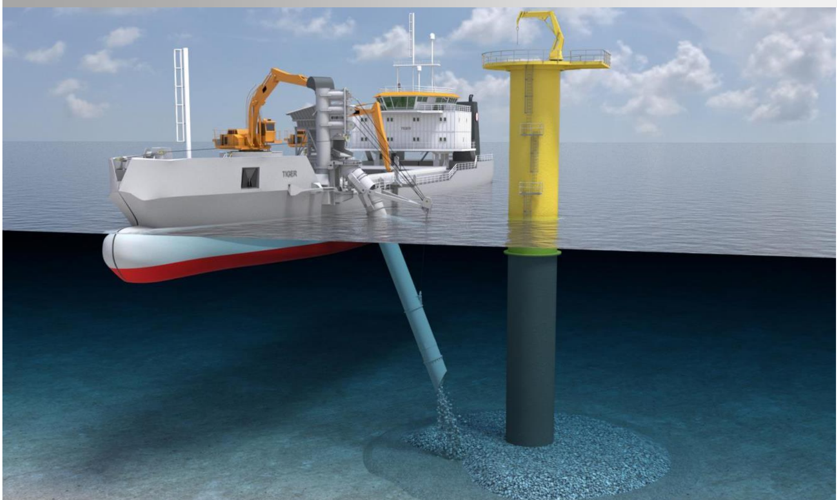
Germany – Installation of Scour Protection for the Butendiek Offshore Wind Farm FPV Tiger
